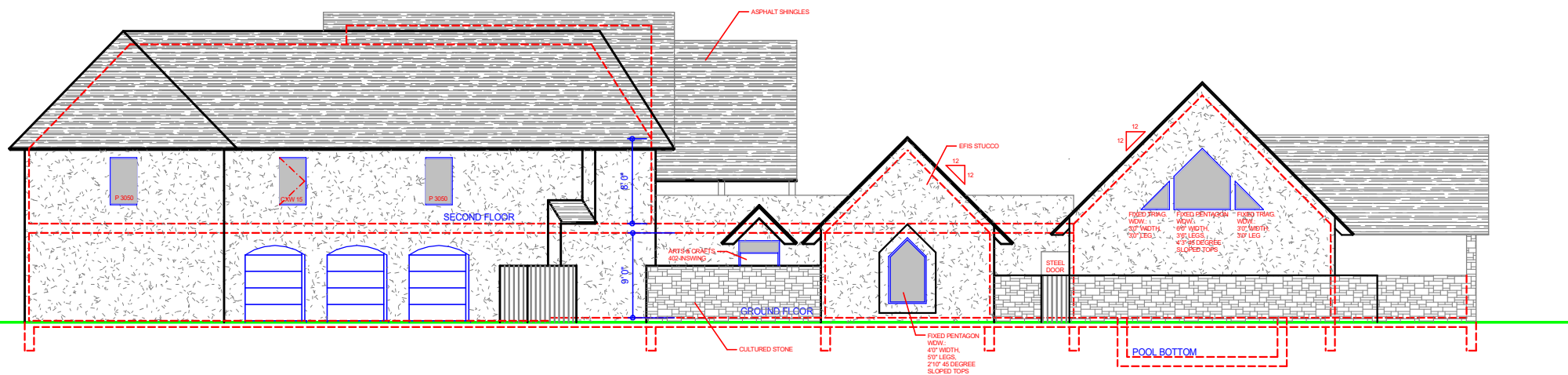
FRONT ELEVATION
