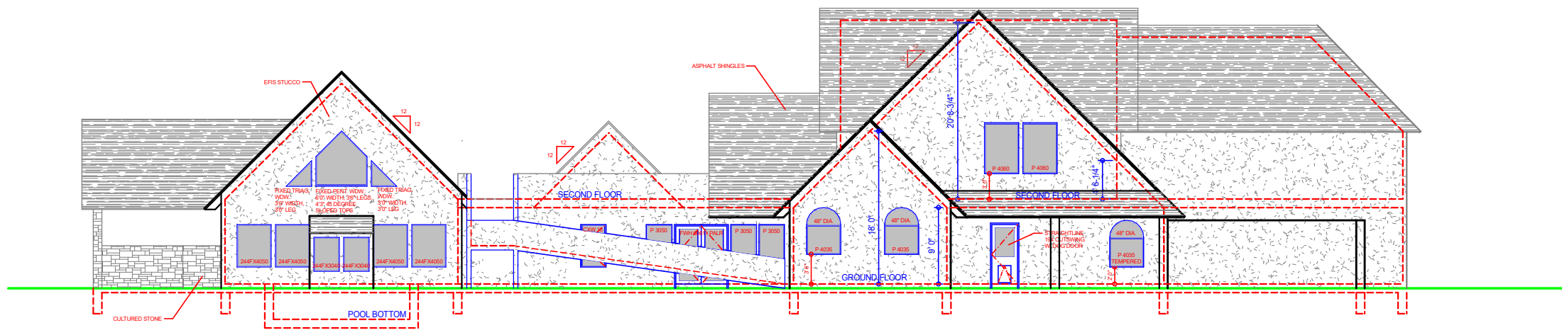
REAR ELEVATION
