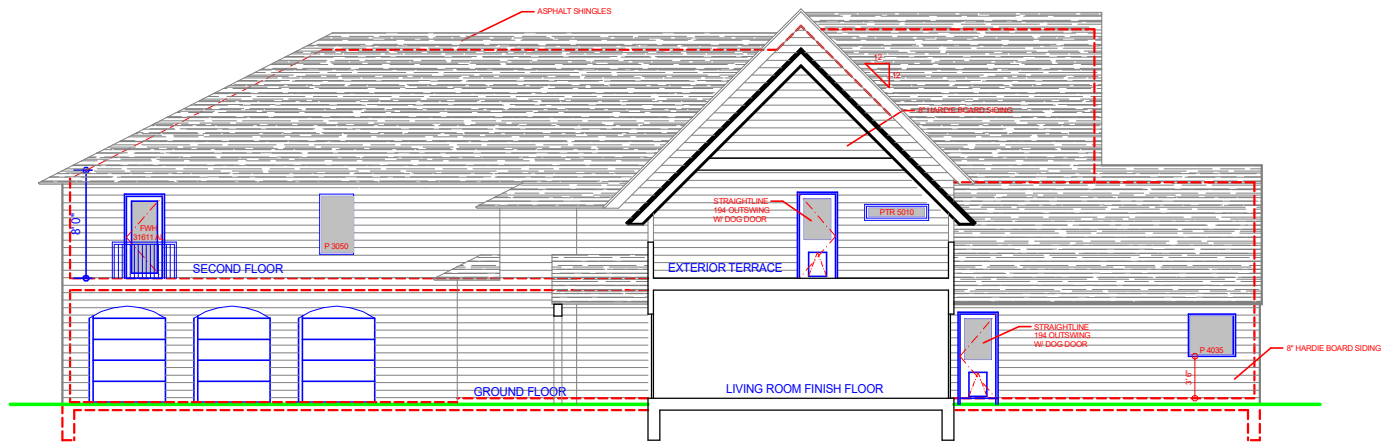
NORTH TERRACE ELEVATION
