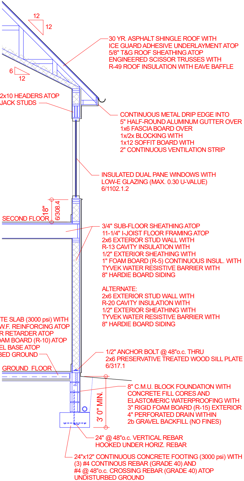
A: TYPICAL WALL SECTION
