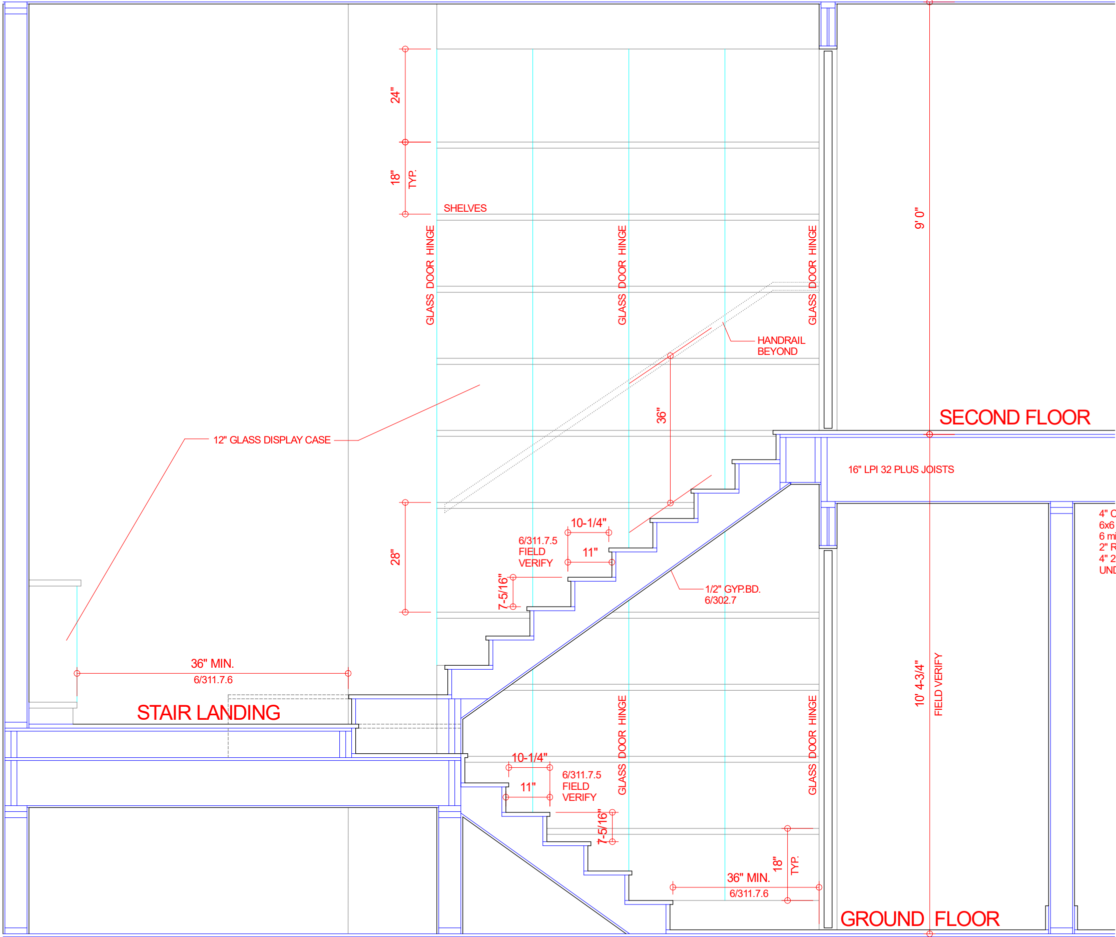
B: STAIR SHOWCASE SECTION
